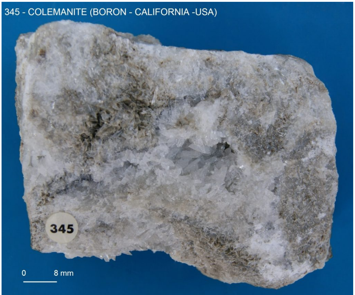
345 - COLEMANITE (BORON - CALIFORNIA -USA)
