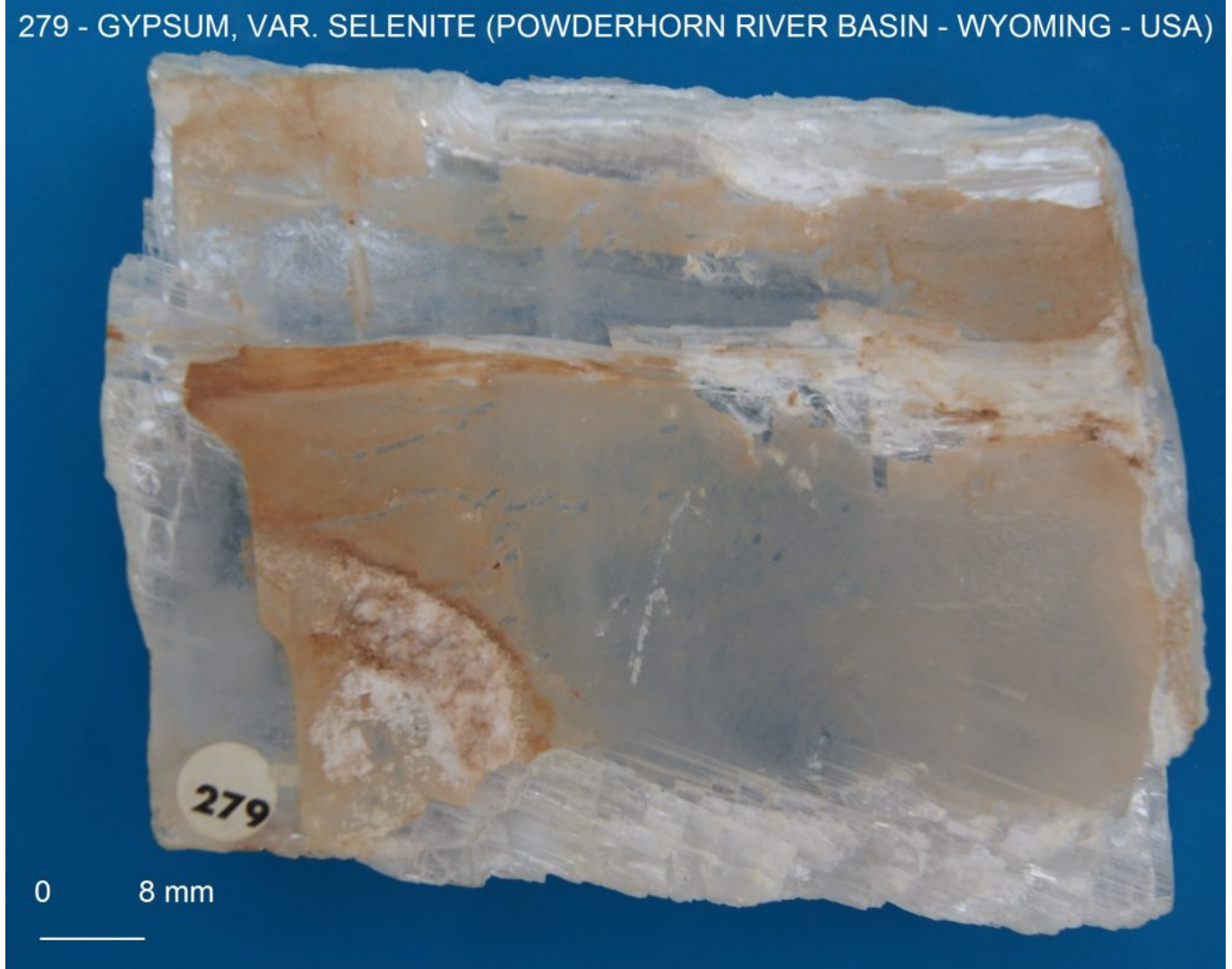
279 - GYPSUM, VAR. SELENITE (POWDERHORN RIVER BASIN - WYOMING - USA)
